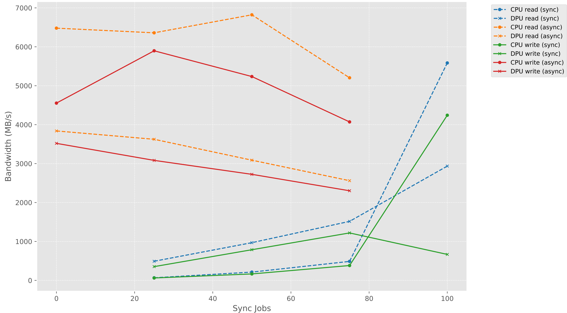
Bandwidth vs Sync Jobs (mixed) - SEQ (CPU vs DPU)
